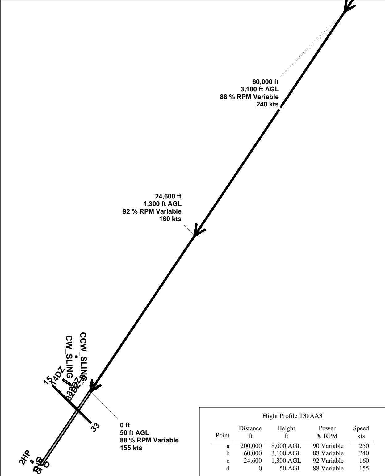
Flight Profile T38AA3 Arrival ~ 3
